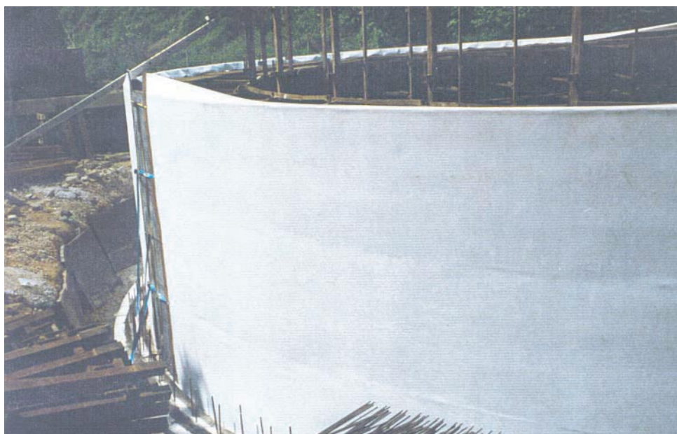
The formwork lined with Formtex ® before casting of a wastewater tank for the sewage work.
